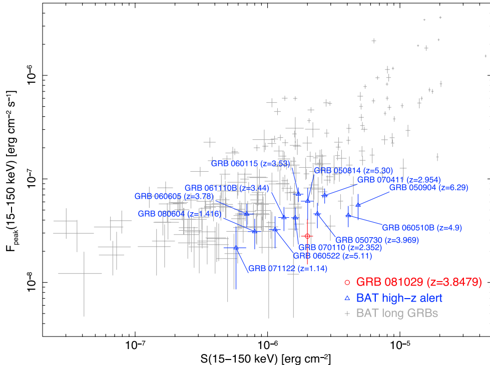
Figure 2. Distribution of the 1 s peak energy flux in the 15–150 keV band vs. the energy fluence in the 15–150 keV band. GRB 081029 is indicated with a red circle. BAT GRBs with known redshifts that satisfy the Ukwatta et al. (2008) high- z criteria are indicated with blue triangles, and BAT long GRBs are shown with gray crosses.
