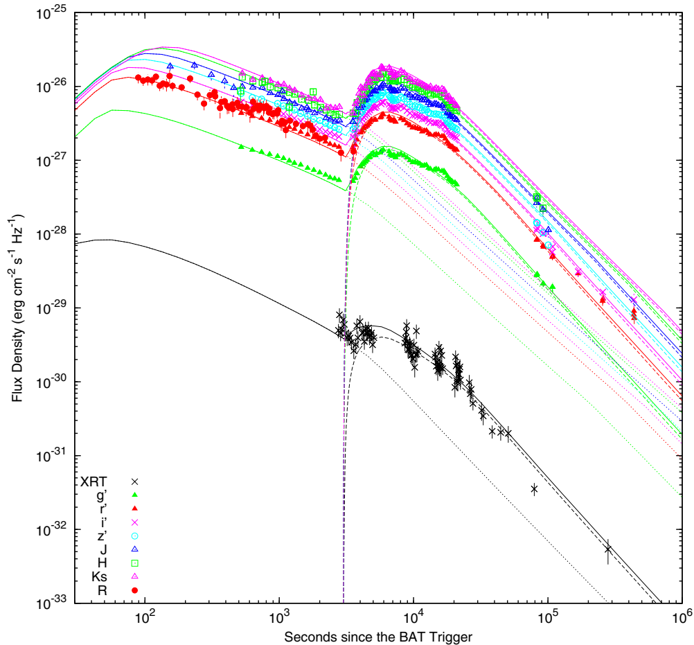
Figure 8. Best-fitting two-component jet model for our light curves. The colors used in the figure are the same as in Figure 5.
