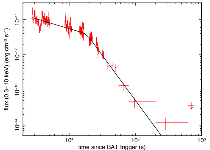
Figure 3. Swift /XRT light curve. The data have not been corrected for Galactic absorption or absorption in the host galaxy.
