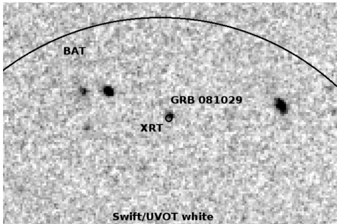
Figure 4. Swift /UVOT white image of the field of GRB 081029. The BAT and XRT error circles are shown. The XRT error circle has a radius of 1''.5 . North is up and east is to the left.
