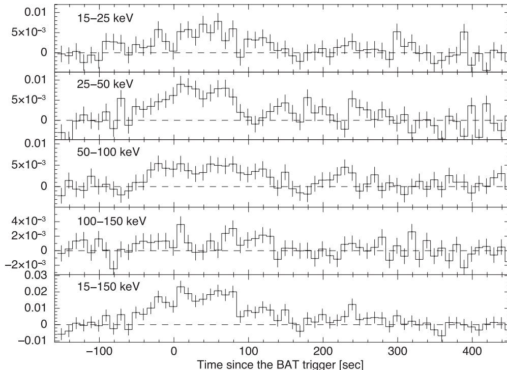
Figure 1. BAT energy-resolved light curves of GRB 081029 with 10 s binning.
