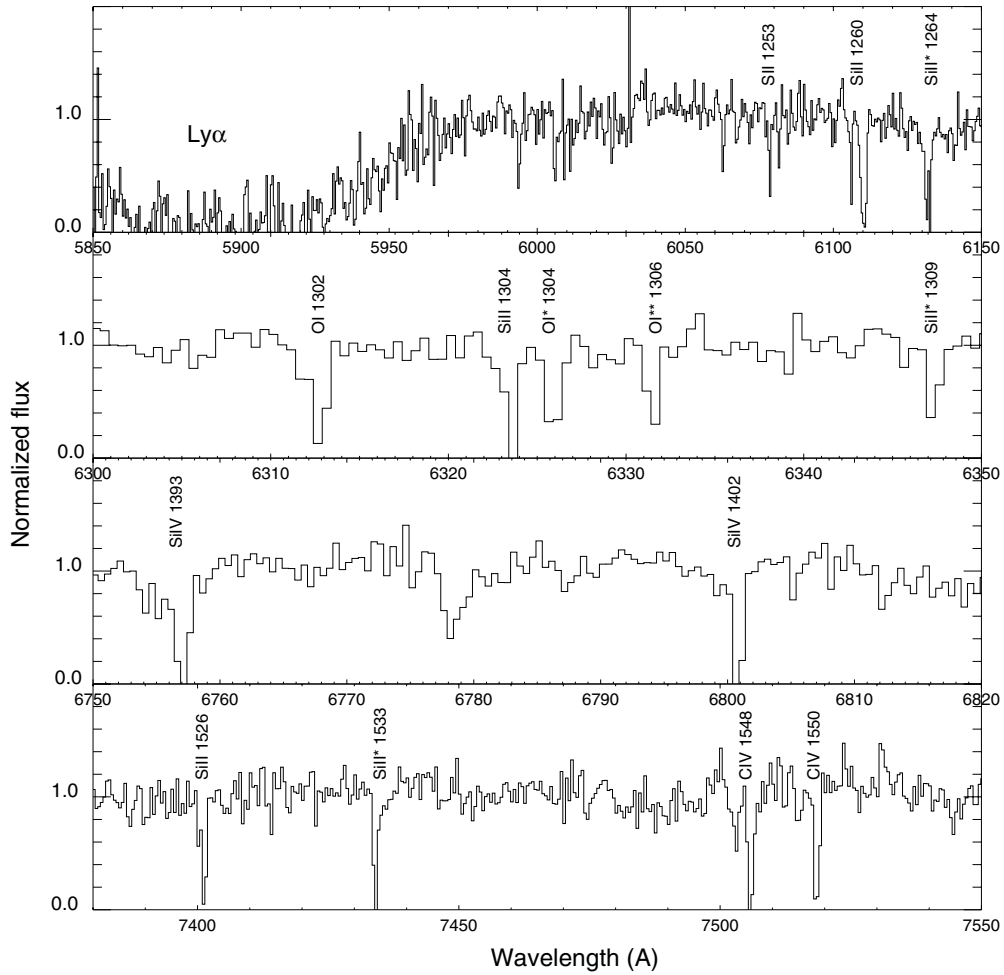
Figure 6. UVES spectrum of the optical afterglow of GRB 081029 showing details of the absorption system.
