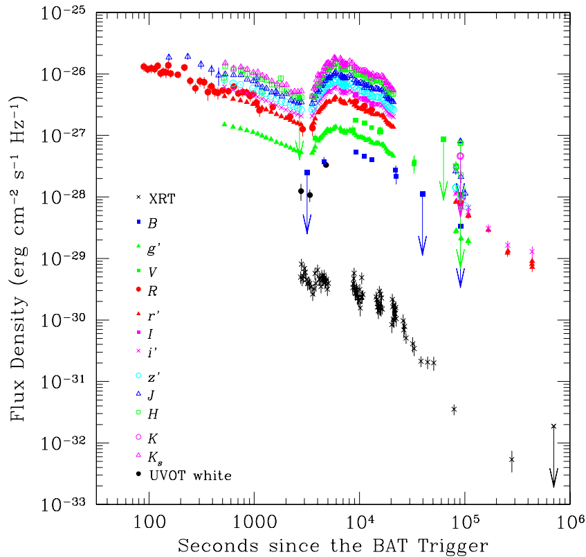
Figure 5. Flux-density light curves for the X-ray data (black crosses) and the optical and infrared data. The optical/infrared photometry has not been corrected for Galactic extinction along the line of sight to the burst, and the X-ray data have not been corrected for Galactic absorption. The vertical bars represent one-sided, 1\sigma error bars in the flux density. In most cases the error bars are smaller than the plotting symbol.
