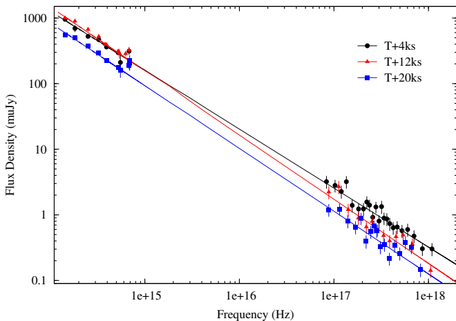
Figure 7. Best-fit model SEDs to the optical, infrared, and X-ray data. The model is the SMC broken power law from Table 5. The fit at 4000 s is shown in black circles, the fit at 12000 s is shown in red triangles, and the fit at 20000 s is shown in blue squares.
