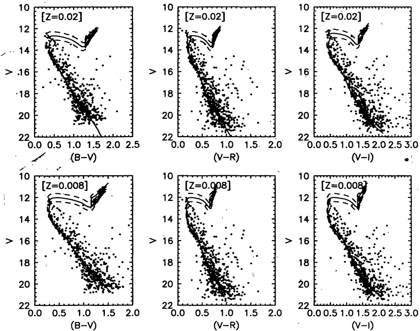
Figure 2. The comparison of theoretical isochrones of Bertelli (1994) for Z=0.02 and Z=0.008 with CMDs of NGC 2309.
