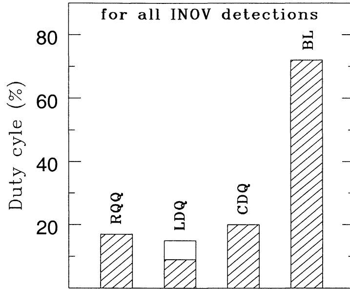
Figure 2. Duty cycle for various classes of AGNs for all variability amplitudes. The shaded bars refer to definite detections of INOV, whereas the non-shaded portion includes the contribution of possible detections of INOV.
