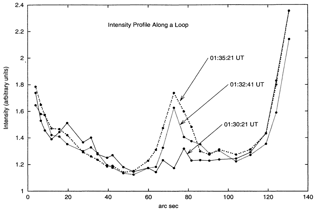
Figure 4. Intensity profile along the third secondary loop for three different times
