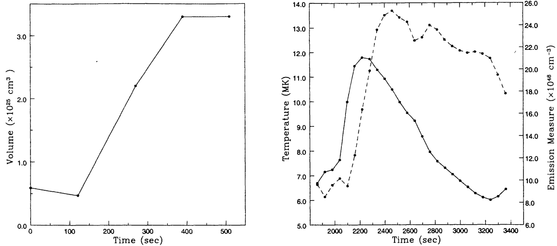
Figure 2. (a) Plot of volume of the flare versus time (Left). (b) Figure on the right shows the plot of temperature (solid line) and emission measure (dashed line) versus time.
