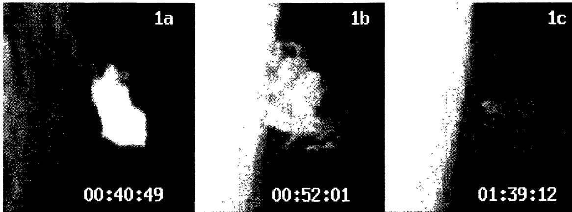
Figure 1. (a) H\alpha filtergram of flare observed from Holloman observatory, New Mexico. (b) and (c) present H\alpha filtergrams of primary and secondary post flare loops observed from State observatory, Nainital. The field of view is 125'' \times 125'' . North is up and west is right.
