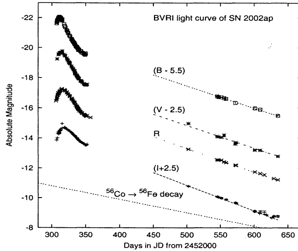
Figure 1. BVRI Photometric Light curves of SN 2002ap Hypernova.
