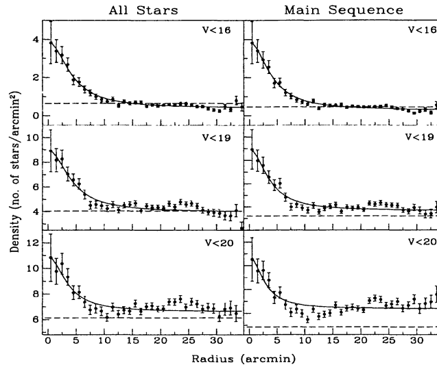
Figure 1. The radial variation of the projected stellar density. Left panel shows distribution of all the stars present in the cluster region. Right panel shows the distribution of stars in the main-sequence band.
