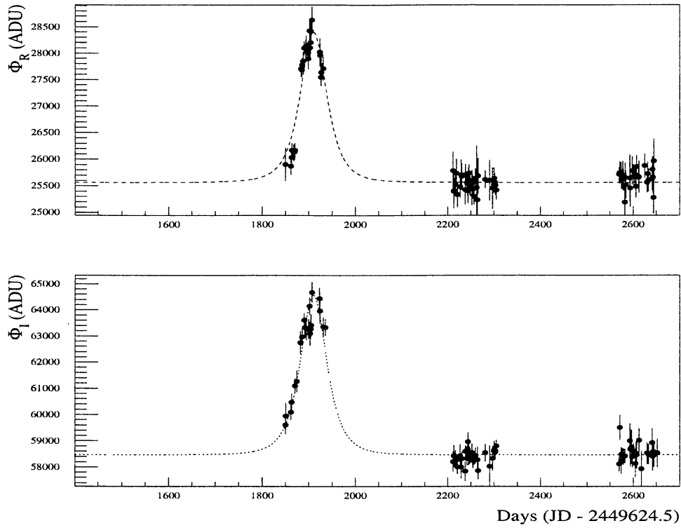
Figure 1. The pixel light curves of a microlensing candidate in both R and I filter detected in our study. The continuous line represent the 7-parameter Paczyński fit.
