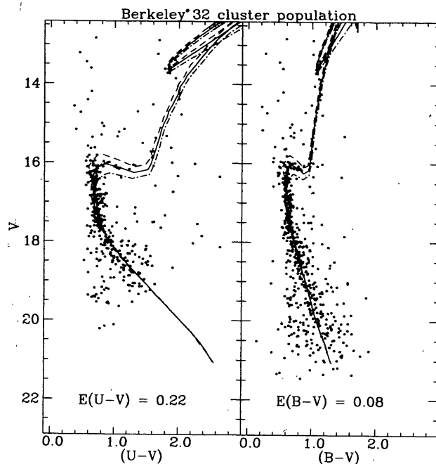
Figure 5. The V , (U - V) and V , (B - V) diagrams generated for the cluster population of Berkeley 32 from the photometric data of Kaluzny & Mazur (1991). The Bertelli et al. (1994) isochrones of the same metallicity and ages, shifted by the same value of the apparent distance modulus as in Fig. 4(B) are shown. The best eye fits to the cluster sequence for the reddening values shown in the plot. The E(U - V) value is not compatible with E(B - V) , including a problem with the U photometry.
