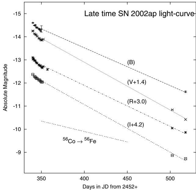
Figure 3. Late time light curve of SN 2002ap. The light curves are offset by a constant value in the magnitude scale, as indicated in the plot. For comparison, slope of the ^{56}\text{Co} \rightarrow ^{56}\text{Fe} decay light curve is also shown.
