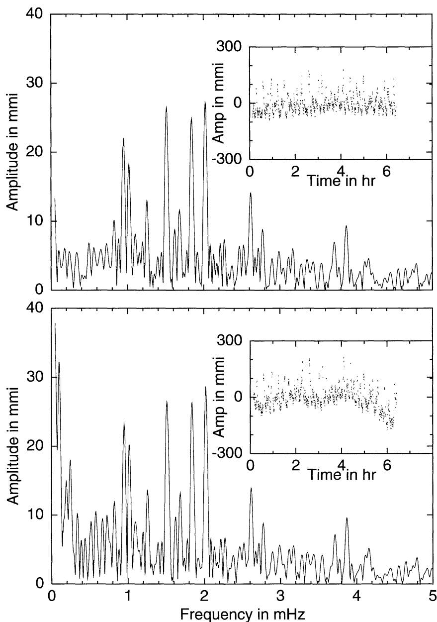
Figure 4. Amplitude spectrum of HL Tau 76.
