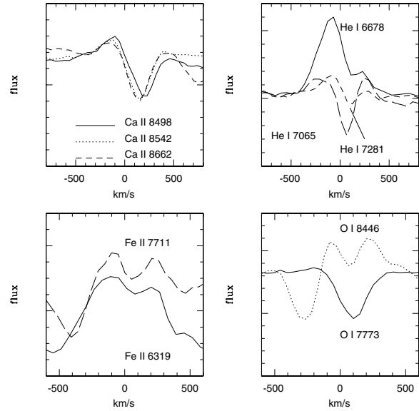
Fig. 13. The line profiles of star S1.
