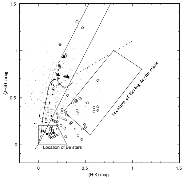
Fig. 18. (J - H) vs. (H - K) colour–colour diagram of stars in the field of NGC 146. The filled circles denote stars for which spectra were obtained. The two H\alpha emission stars are denoted by dots with a circle around them. The filled triangles are the PMS stars with high extinction. The symbol star denotes objects that are located to the right of the PMS isochrones. The MS and the giant star locations in the CMD are shown (Bessell & Brett 1988). The location of T-Tauri stars are shown as the dashed straight line (Meyer et al. 1997). The location of Be stars is taken from Dougherty et al. (1994) and the location Herbig Ae/Be stars is taken from Hernandez et al. (2005).
