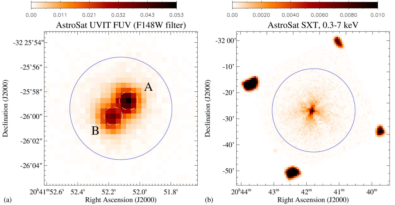
Figure 1. UV (a) and X-ray (b) images of AT Mic from the AstroSat UVIT FUV and SXT observations on 2018 October 3–4, for the entire observation intervals. The color bars are in units of counts s -1 pixel -1 . The blue or white circles indicate the extraction regions for light curves and spectra.
