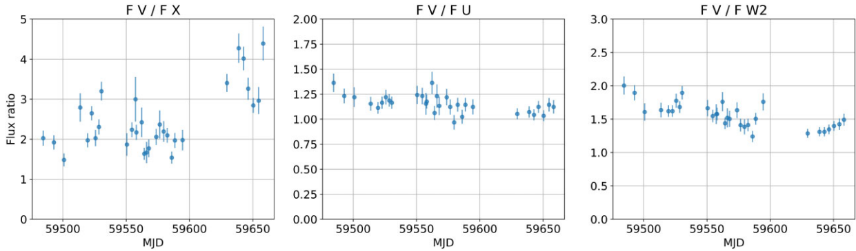
Figure 6. Spectral ratios between the visual flux F_V , near-ultraviolet flux F_U , far ultraviolet flux F_{W2} , and X-ray flux F_X , extracted from the Swift data. The flare, visible in F_V/F_X plot, occurs at \sim JD2459638 and this epoch is fairly close to the secondary SMBH disc impact in our description. In our model, we associate its origin to the plasma, ejected from the disc by the impact of the secondary SMBH, that may have eventually produced the bremsstrahlung flare during 2022 July–August. The other ratios are consistent with this being an UV dominated flare.
