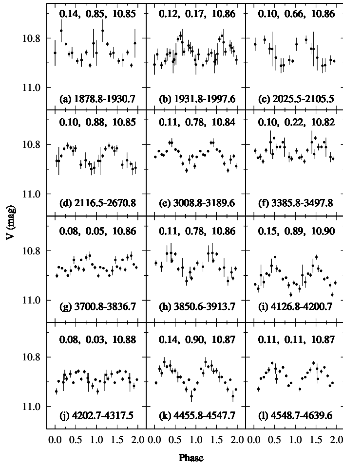
Fig. 2 V -band folded light curves of CV Cha at different epochs of ASAS observations. The observing duration is given at the bottom of each panel in JD ( =2450000.0+ ). Parameters derived from the light curve are mentioned in the sequence amplitude, phase minimum and mean V -band magnitude at the top of each panel.
