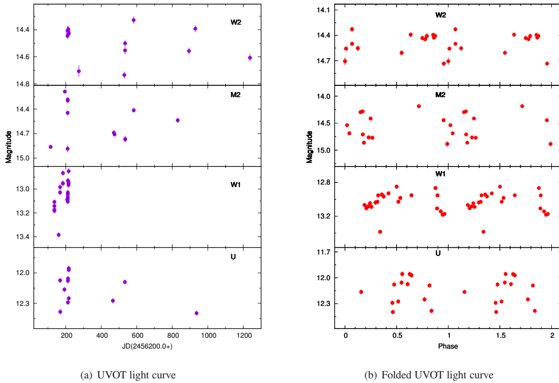
Fig. 4 (a) UVOT light curves of CV Cha as obtained from Swift . (b) Phase folded UVOT light curve of CV Cha. The central wavelengths of U , W1 , M2 and W2 filters are 3465, 2600, 2246 and 1928 Å, respectively.
