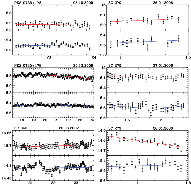
Figure 5. As Fig. 1, but for PKS 0735+178, 3C 279 and 3C 345.
